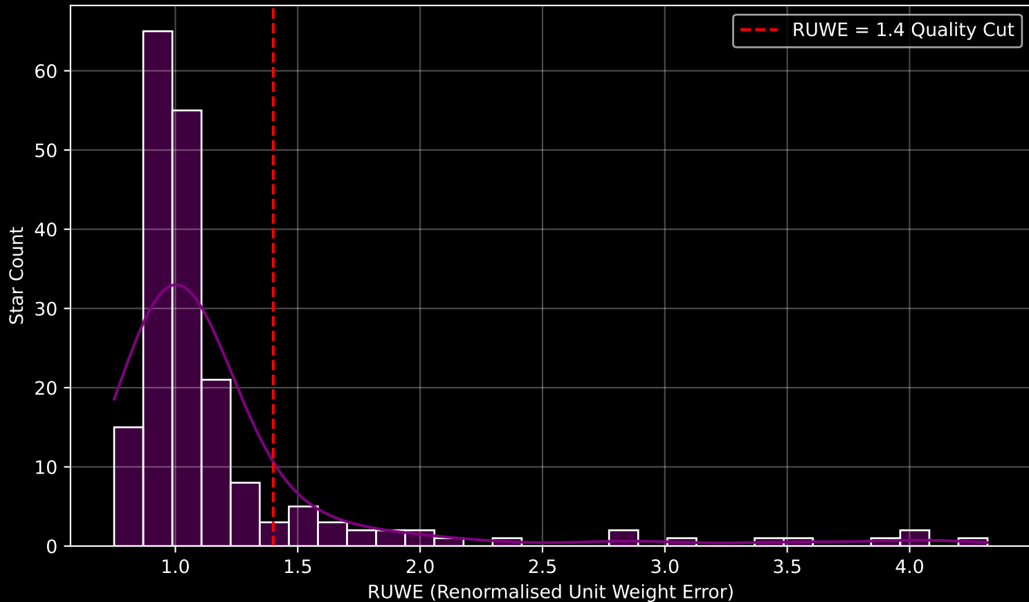
GAPOGEE DR17 Field [091-43_MGA] RUWE Distribution (n= 192)
