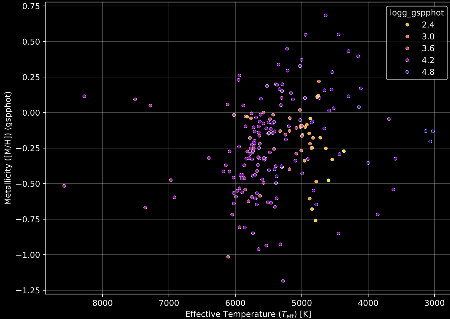
APOGEE DR17 Field: [091-43_MGA] Stellar Population Parameters (n= 202)
