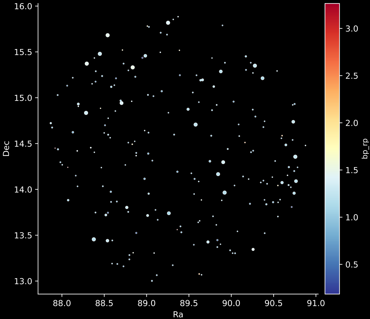
APOGEE DR17 Field: [091-43_MGA] Stars: 202
