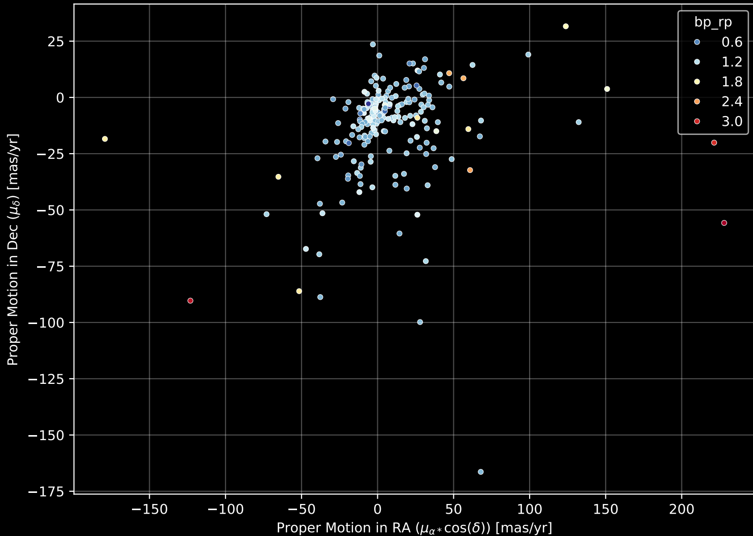
APOGEE DR17 Field: [091-43_MGA] Proper Motion Diagram (n= 202)
