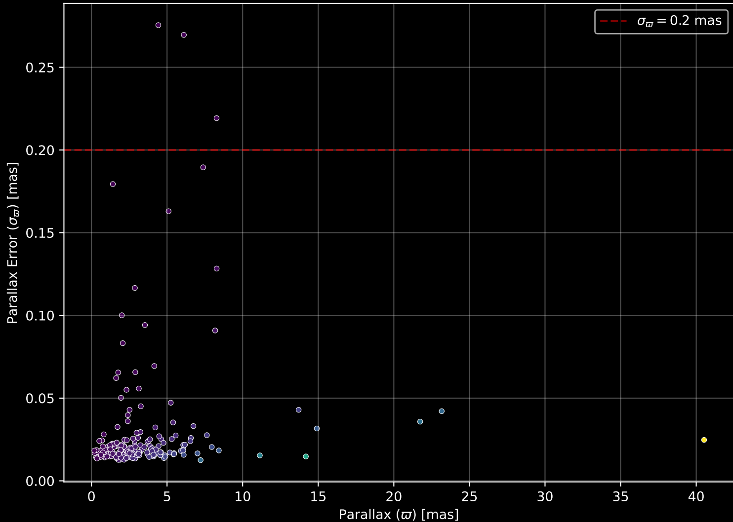
APOGEE DR17 Field: [091-43_MGA] Parallax Quality (n= 202)
