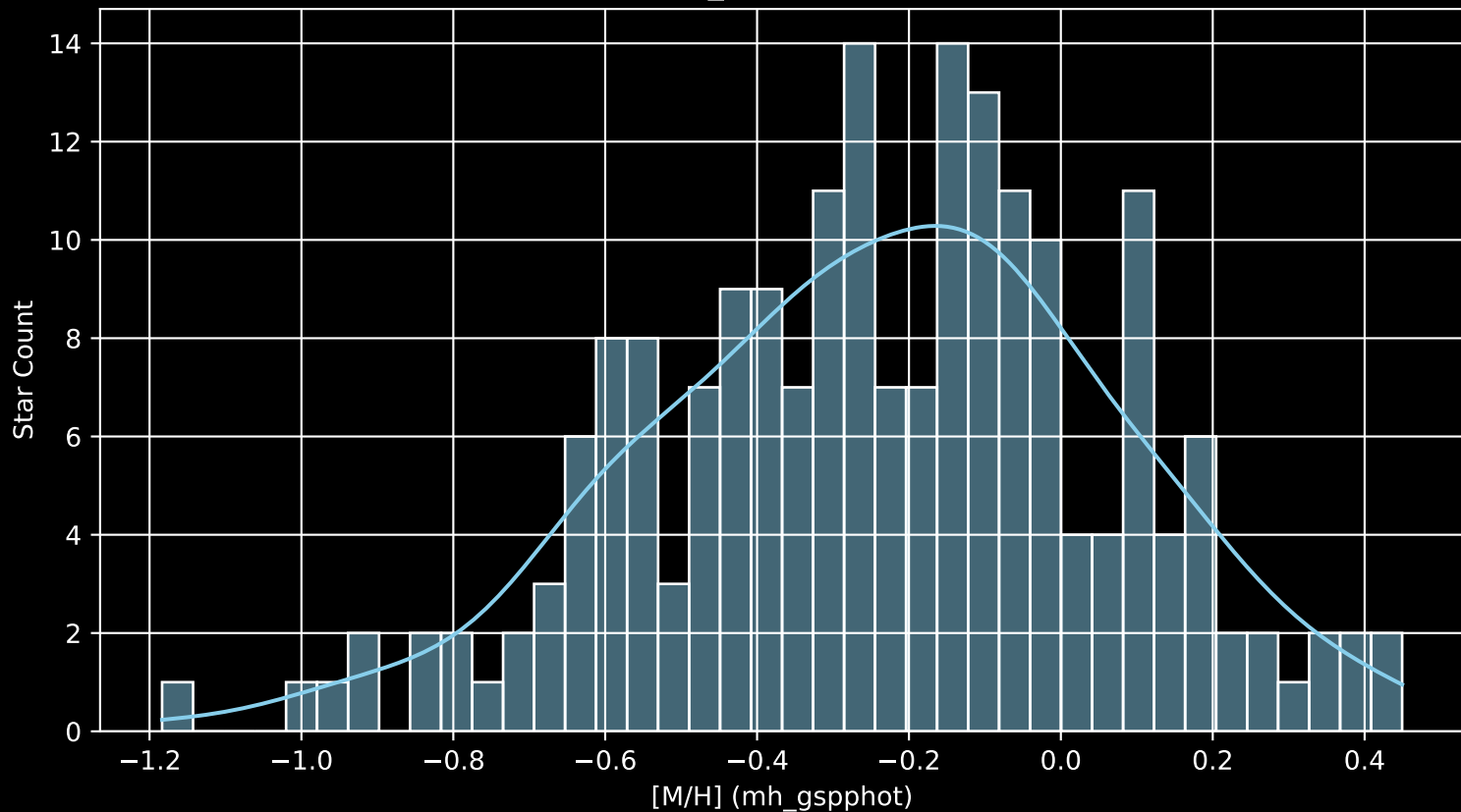
APOGEE DR17 Field: [091-43_MGA [M/H] (mh_gspphot) (n= 199)
