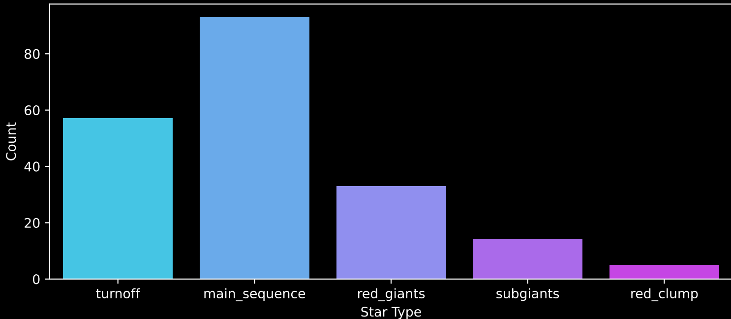
APOGEE DR17 Field: [091-43_MGA] Count plot of Star Type
